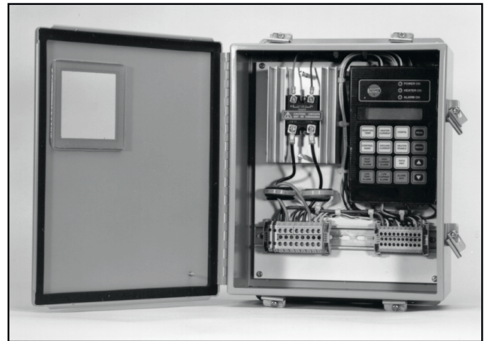
TC 201a mounted in a NEMA 4 painted steel enclosure
